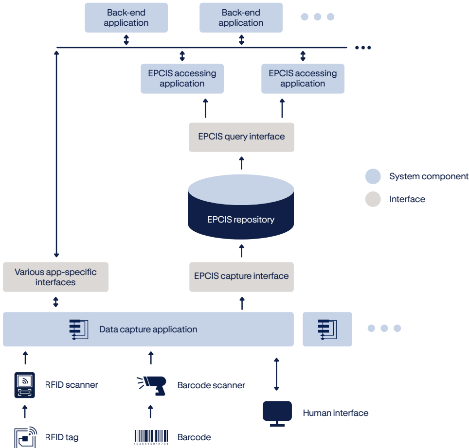
Figure 3: EPCIS tech components
